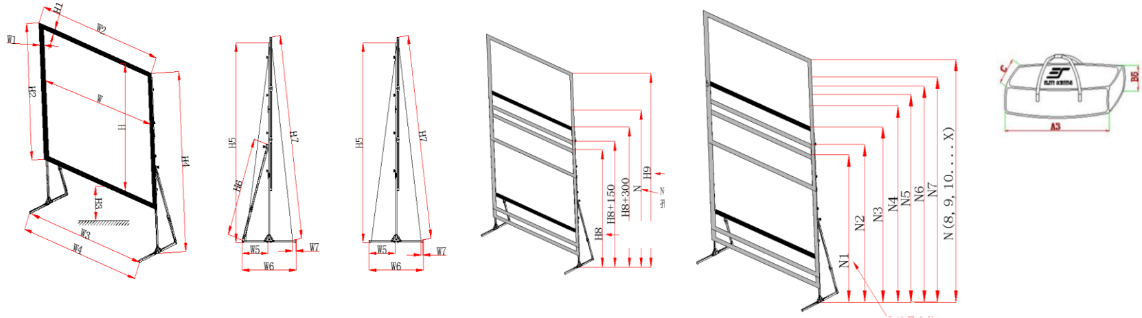
120" and Below: No AT Leg
