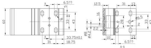
Wall/Ceiling Brackets Unit of measure: mm
