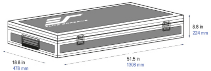
Aluminum Case for Models 150", 180" and 200"
