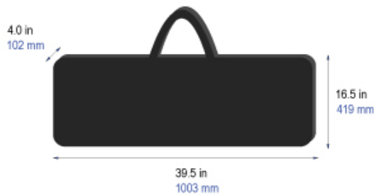
Cloth Carrying Bag for models 100" and 120"
