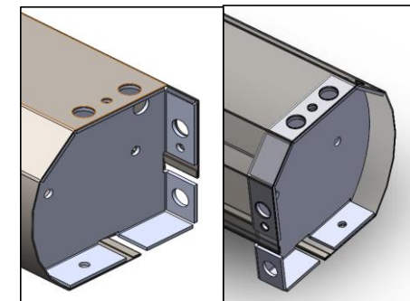
Case for 125" Models and Above
