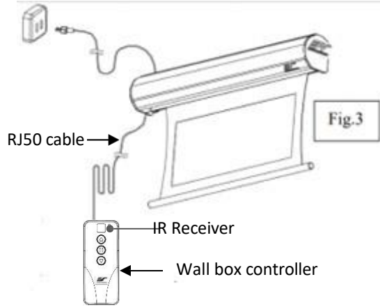
Wall box controller BACK VIEW
