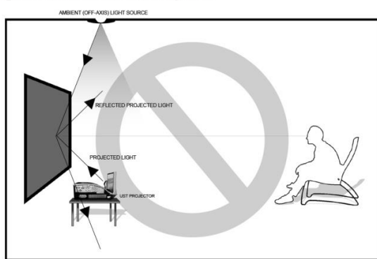
ULTRA SHORT THROW PROJECTOR ILLUSTRATION (NOT COMPATIBLE)
